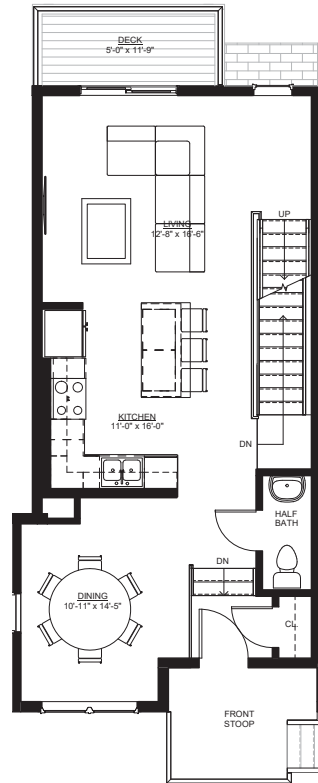
② #31 FIRST FLOOR
