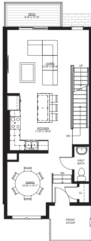
② #27 FIRST FLOOR
