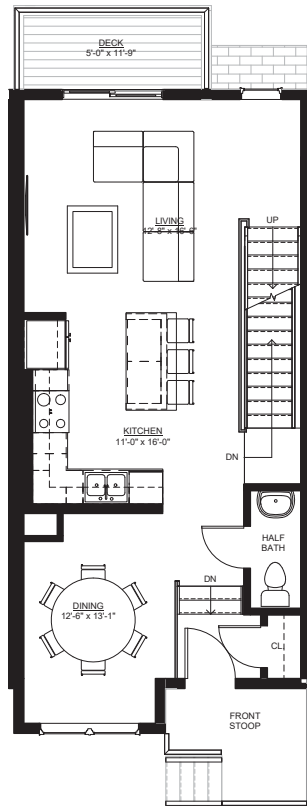
② #25 FIRST FLOOR
