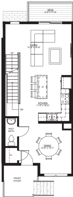
② #19 FIRST FLOOR
